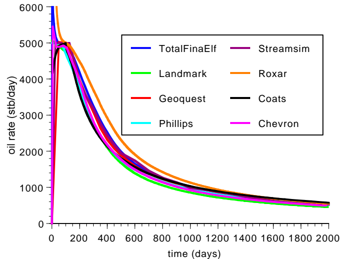
Fig 13: Comparison of All Field Oil Rate Curves for Model 2
