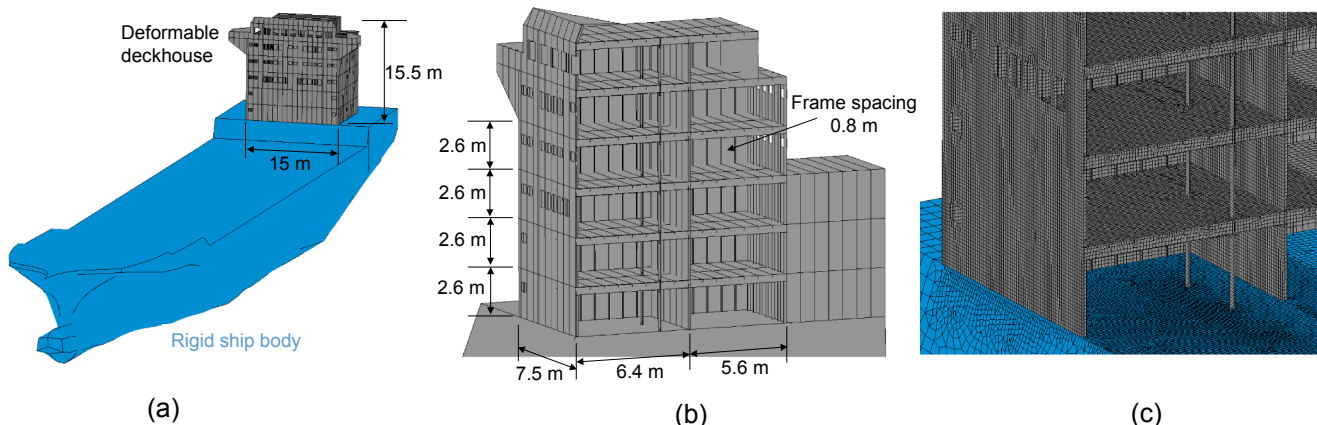
Fig. 3. (a) Container ship model, (b) detailed deckhouse modelling, and (c) mesh illustration.
